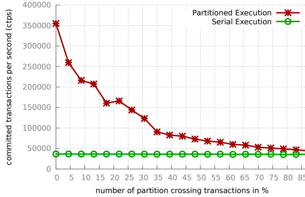
Figure 1: The performance in the TPC-C benchmark while varying the number of partition-crossing transactions
