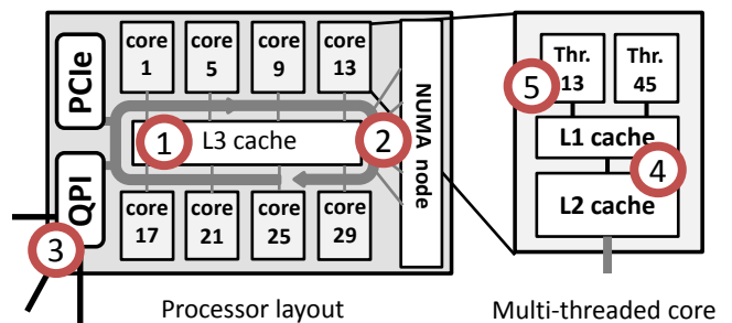
Figure 1: An Intel SandyBridge architecture depicting shared DRAM resources for programs: (1) the last level cache, (2) local DRAM bandwidth, (3) interference on the QPI interconnect, (4) sharing of the private L1 and L2 caches, and (5) sharing a hardware thread.
