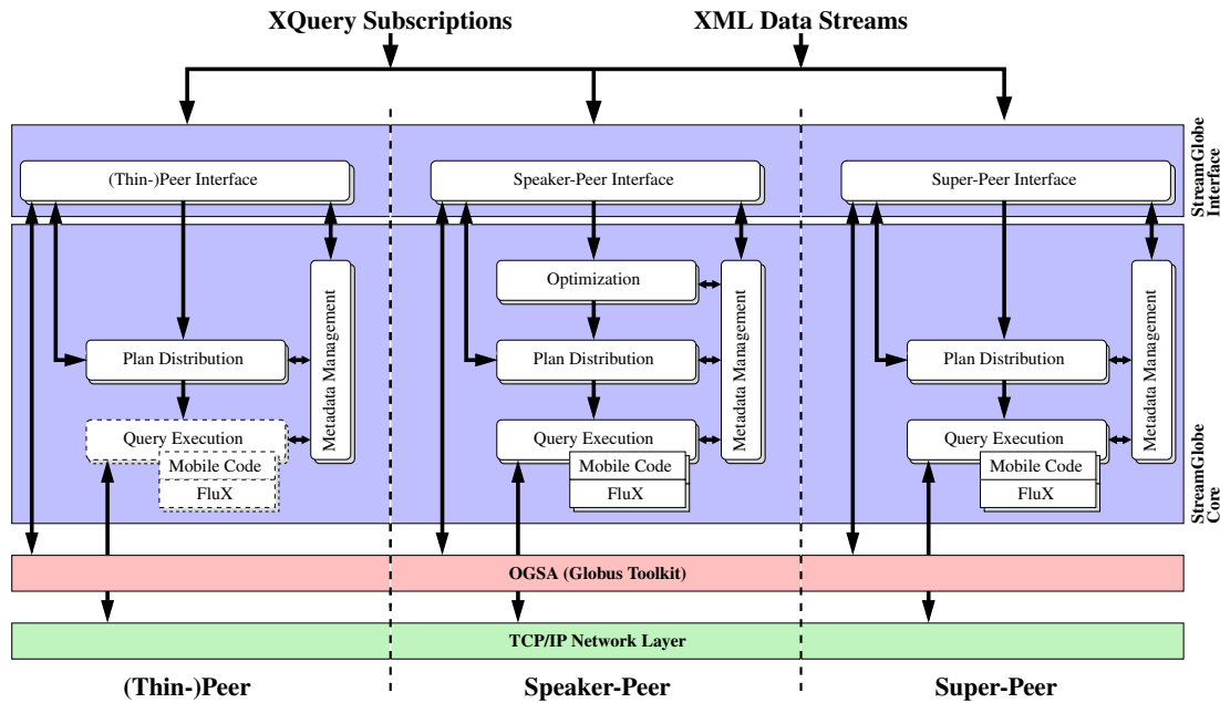
Figure 3: Architecture Overview
