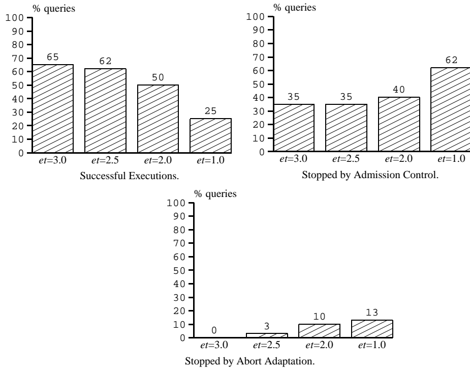
Fig. 25. The Success of Queries with different et Values.
