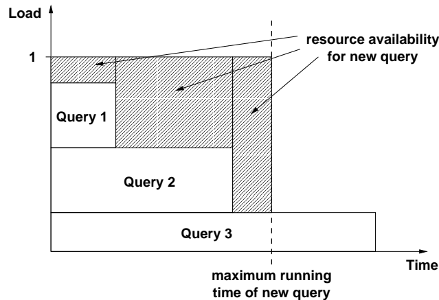
Fig. 11. Gathering Available Shares on a Resource During Admission Control
