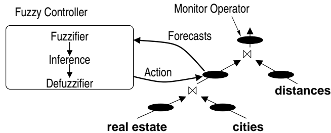
Fig. 14. Feedback Loop for QoS Adaptations.
