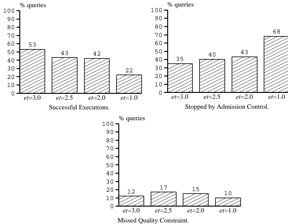
Fig. 23. The Success of Queries for different et values with Admission Control activated.
