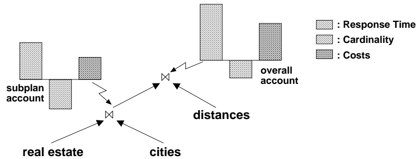
Fig. 12. QoS Accounts of a Query Plan.
