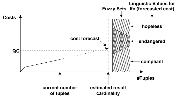
Fig. 15. Mapping Quality Parameter Forecasts on Fuzzy Sets.
