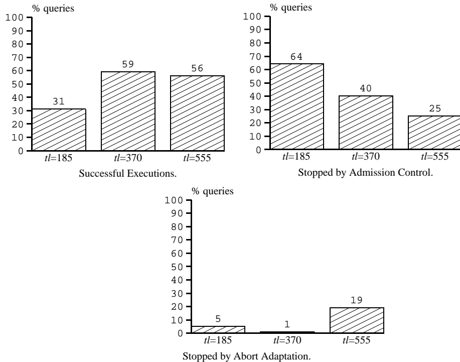
Fig. 26. The Success of Queries with different Time Limits.
