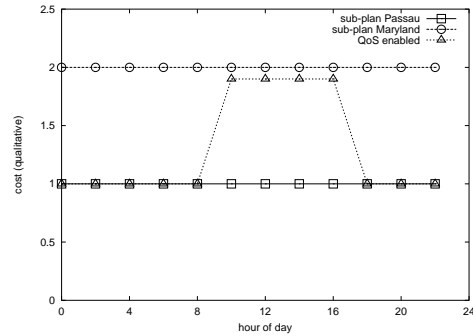
Fig. 19. Qualitative View on the Wrapper Experiments.
