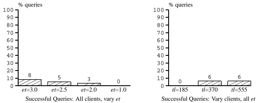
Fig. 22. The Success of Queries with no QoS Techniques applied.
