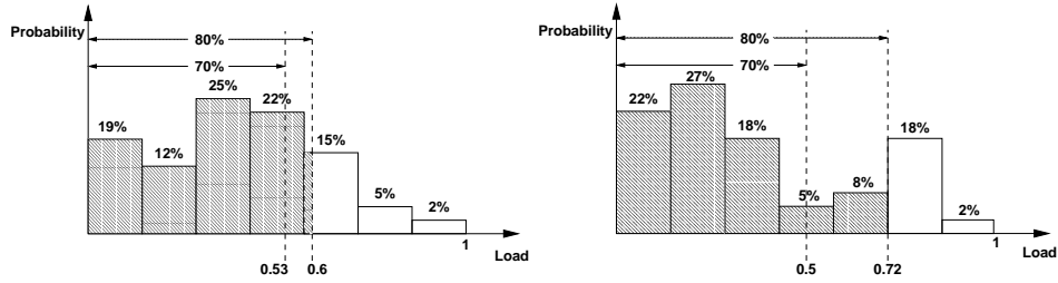
Fig. 6. Load Distribution of different Cycle Providers.
