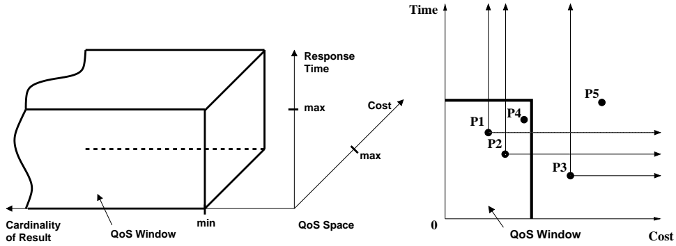
Fig. 7. The QoS Space and the QoS Window. Fig. 8. The Partial Order for Plans.
