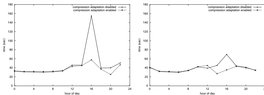
Fig. 20. Executing a remote Scan Operation on Day 1. Fig. 21. Executing a remote Scan Operation on Day 2.
