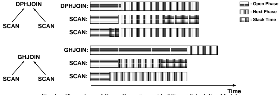
Fig. 4. Chronology of Query Executions with different Scheduling Models
