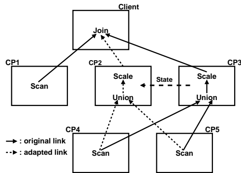
Fig. 13. Moving a Plan Fragment from one Cycle Provider to another.
