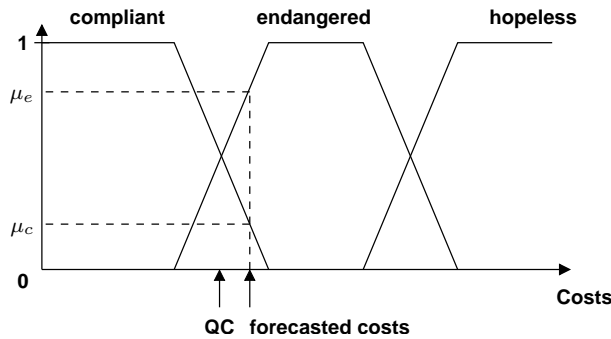
Fig. 16. The Fuzzy Sets for the Cost Forecast Value..
