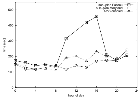
Fig. 17. Retrieving Data through Wrappers on Day 1. Fig. 18. Retrieving Data through Wrappers on Day 2.
