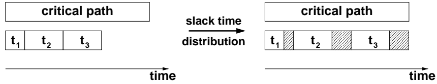
Fig. 10. Slack Time Distribution
