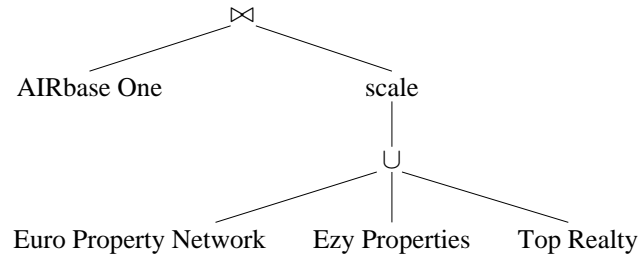
Fig. 1. Query Evaluation Plan for the Example Query
