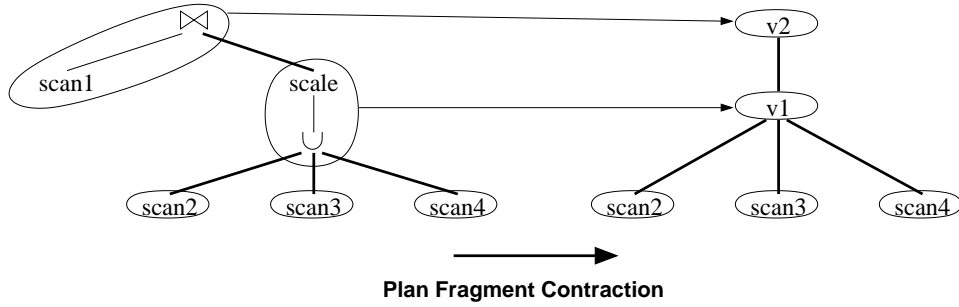
Fig. 5. Fragmentation of QEPs in Parallel Working Plan Fragments.
