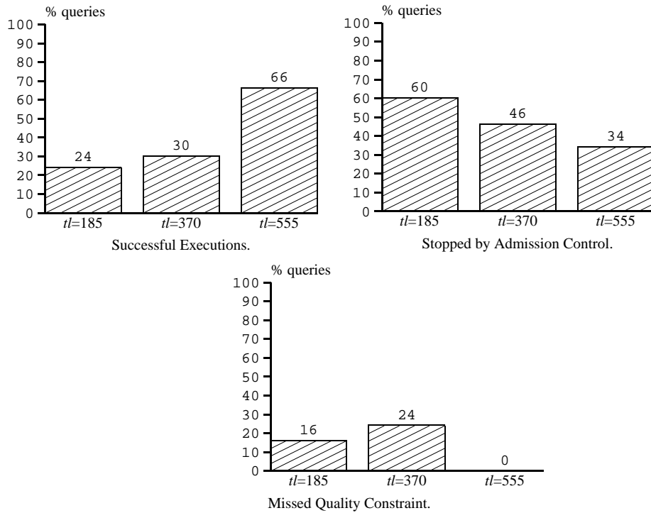
Fig. 24. The Success of Queries for different tl values with Admission Control activated.
