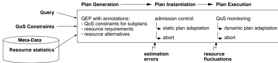
Fig. 2. The Interaction of Query Processing and QoS Management
